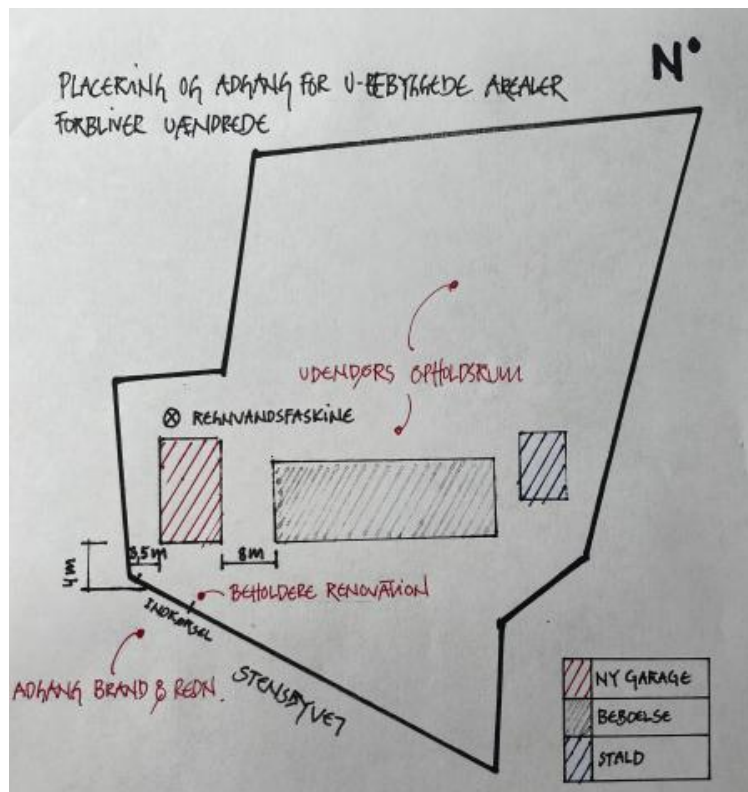
Figur 2. Situationsplan for nye forhold.
