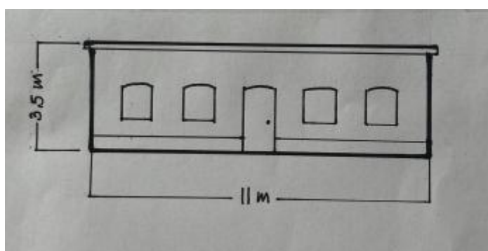
Figur 5. Facade tegning (øst).
